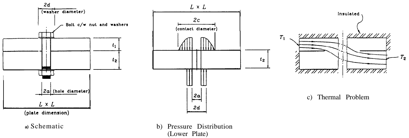
Figure 1: Bolted Joint
